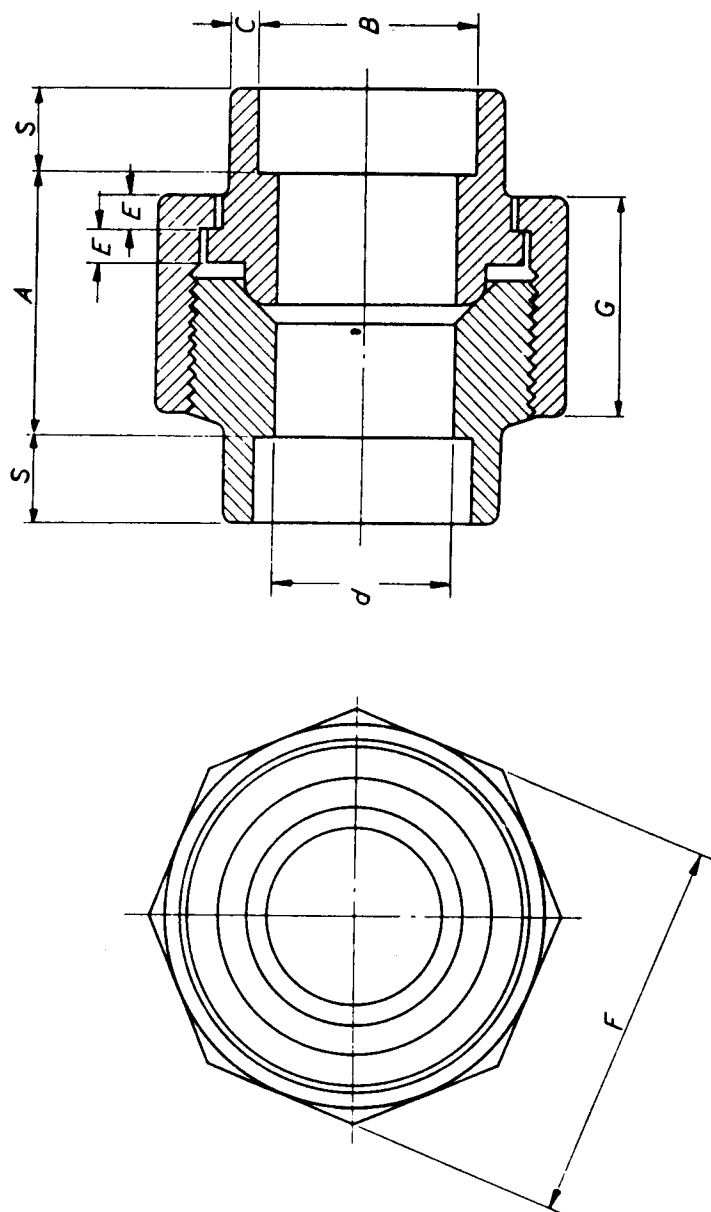
Socket-welding fittings. Dimensions of unions
