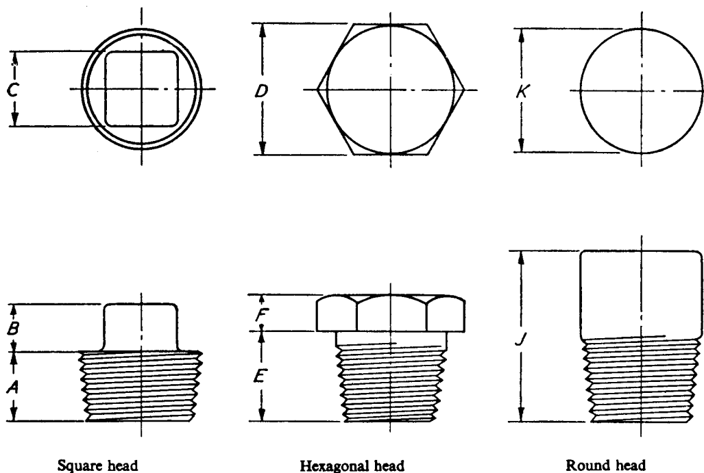
Screwed fittings. Minimum dimensions of pipe plugs
