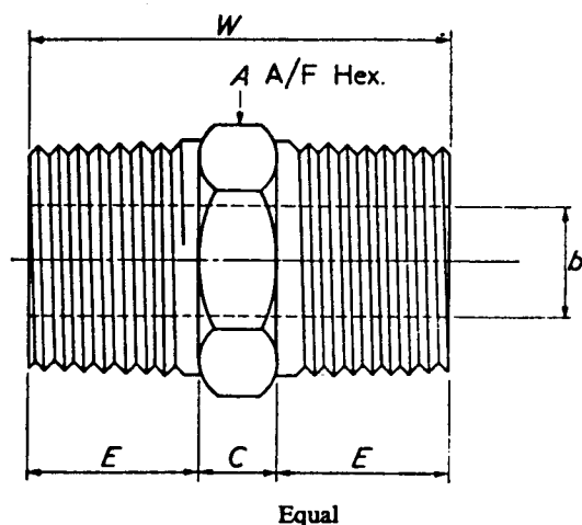
Screwed fittings. Dimensions of hexagonal nipples
